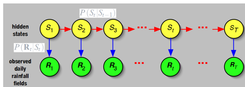
FIGURE A.4. GENERAL STRUCTURE AND EVOLUTION OF HMM
