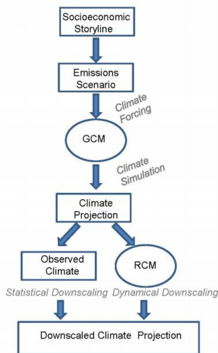
FIGURE I. ILLUSTRATION OF THE COMPONENTS INVOLVED IN DEVELOPING GLOBAL AND REGIONAL CLIMATE PROJECTIONS
