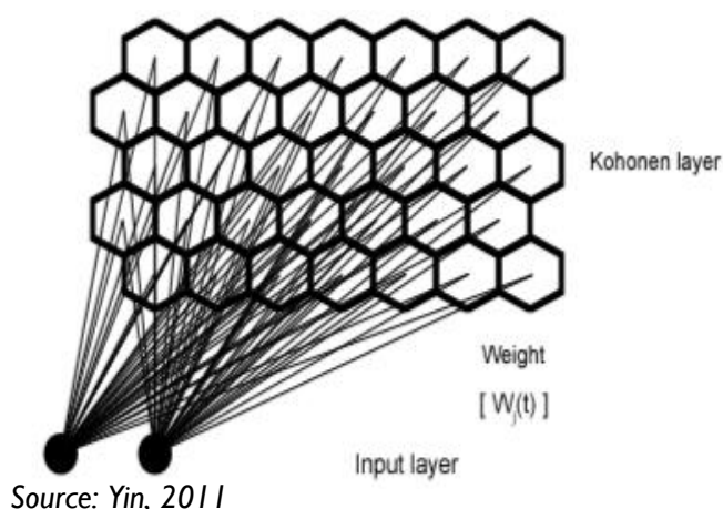
FIGURE A.3. STRUCTURE OF TWO DIMENSIONAL SELF-ORGANIZING MAP
