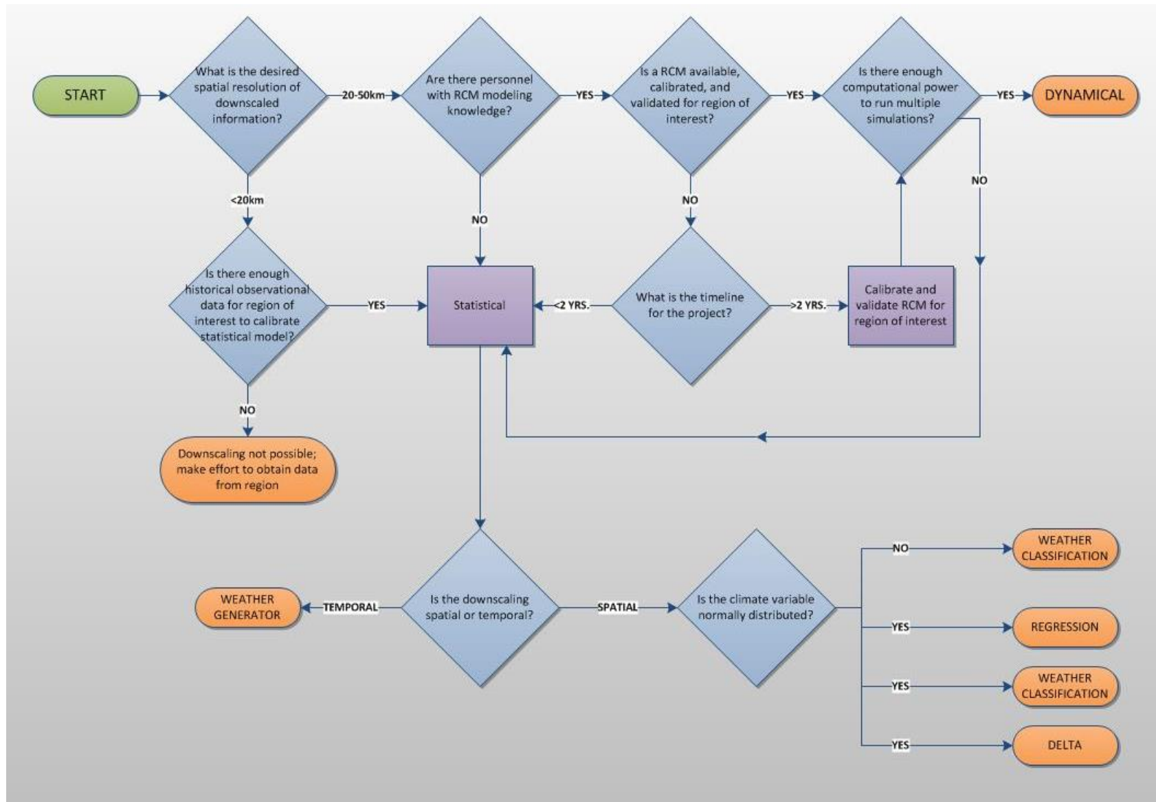
FIGURE 2. WHICH DOWNSCALING TECHNIQUE IS MOST APPROPRIATE FOR THE PRESENT STUDY?
