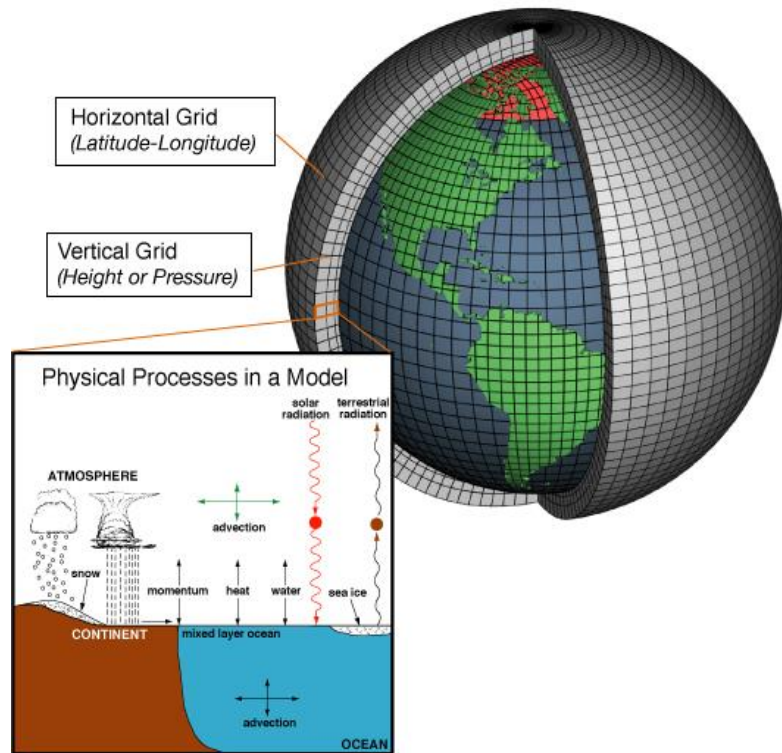
FIGURE 3. CONCEPTUAL STRUCTURE OF A GCM
