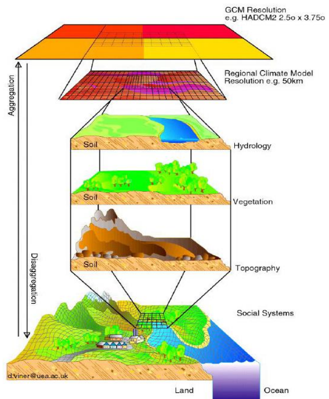
FIGURE 4. THE CONCEPT OF SPATIAL DOWNSCALING
