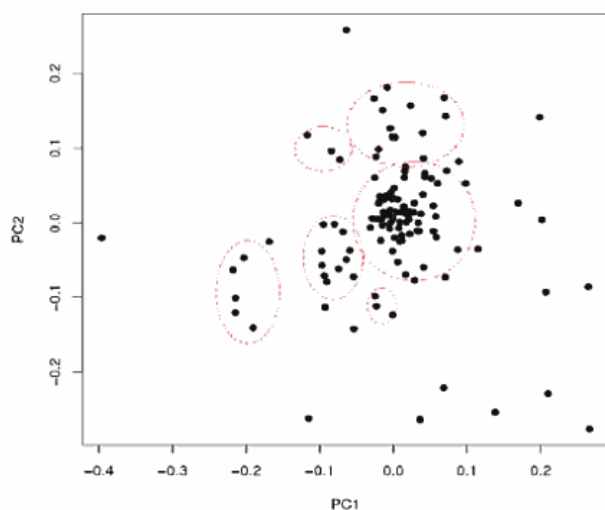
FIGURE A.1. CLUSTER ANALYSIS
