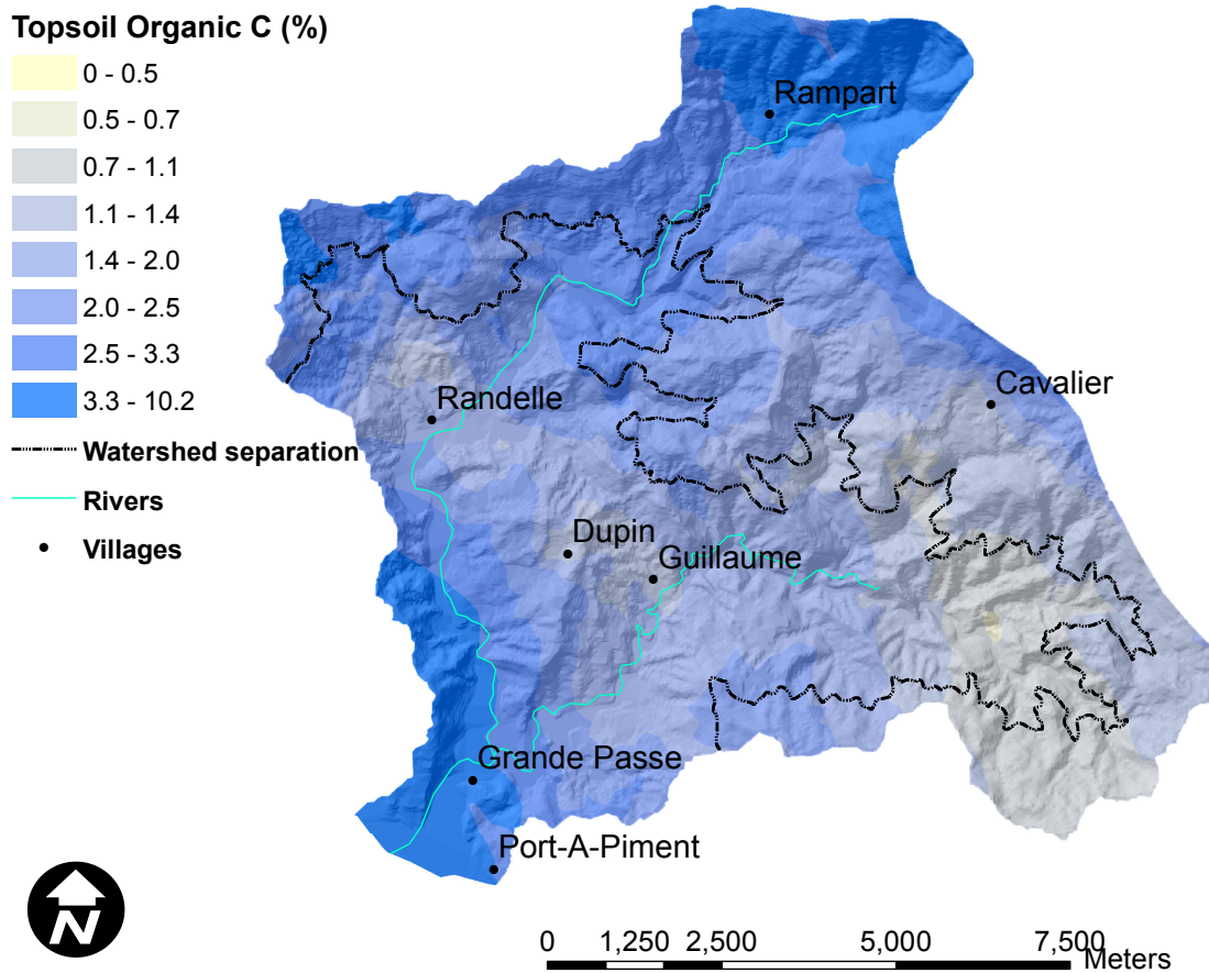
Map 19 Estimated map of Organic Carbon (OC) concentrated in topsoil for Port-à-Piment Watershed
